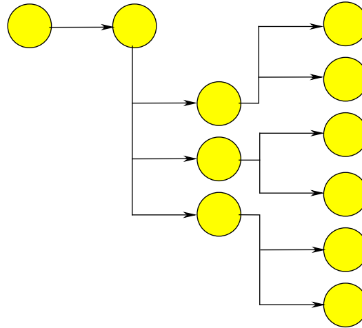
Combinatoric
