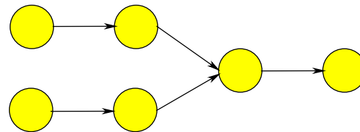
Convergent (Y)
