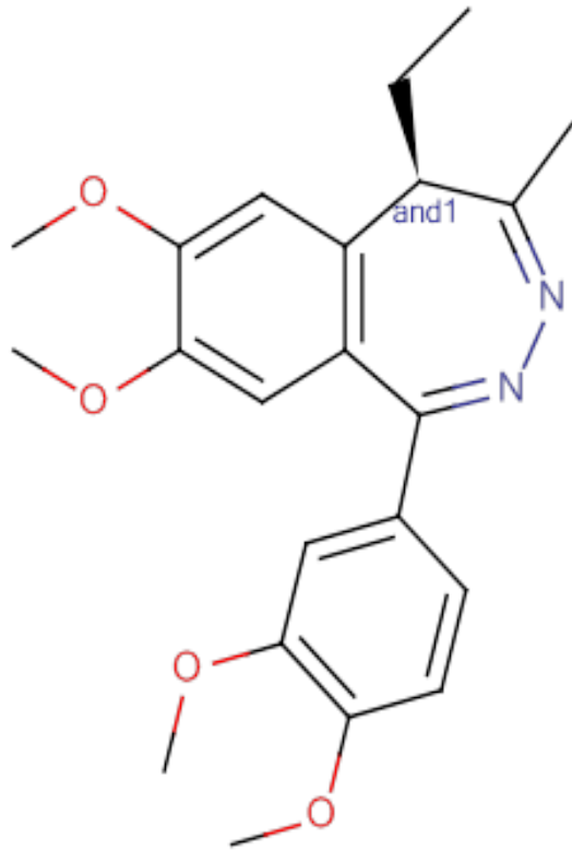
RACEMIC
