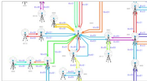
Network Topology
